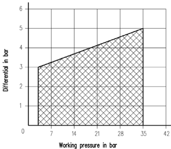
DIFFERENTIAL PRESSURE OF IPH-350 PRESSURE SWITCH
