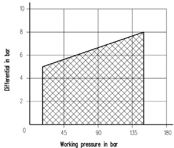
DIFFERENTIAL PRESSURE OF IPH-630 PRESSURE SWITCH
